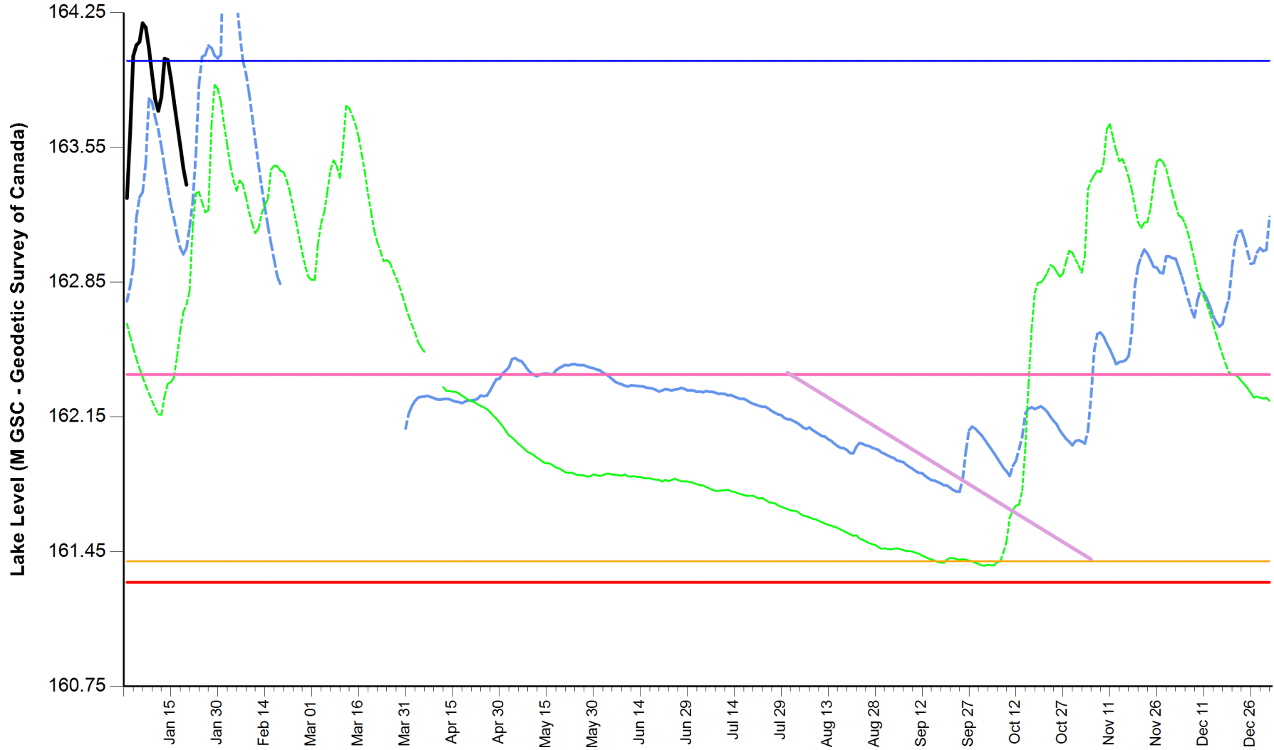
2021 Cowichan Lake Level - 2021 (Black) & 2020 (Blue) & 2016 (Green)
